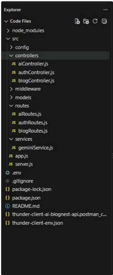
Server/ project structure as committed to the repository.
